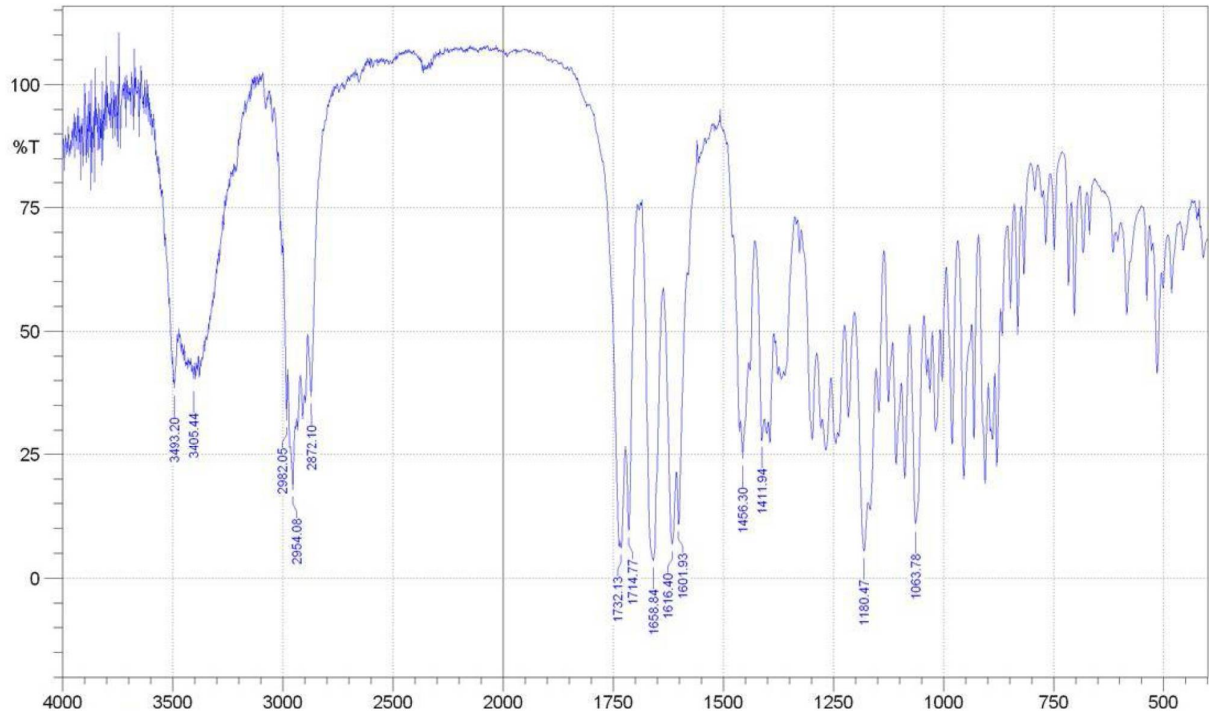
Dihydrocortisone
